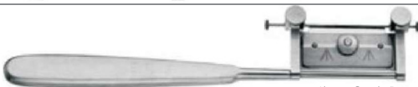
Item Code Description 09-D-08 SILVER DERMATOME, 19CM, ADJUSTABLE
